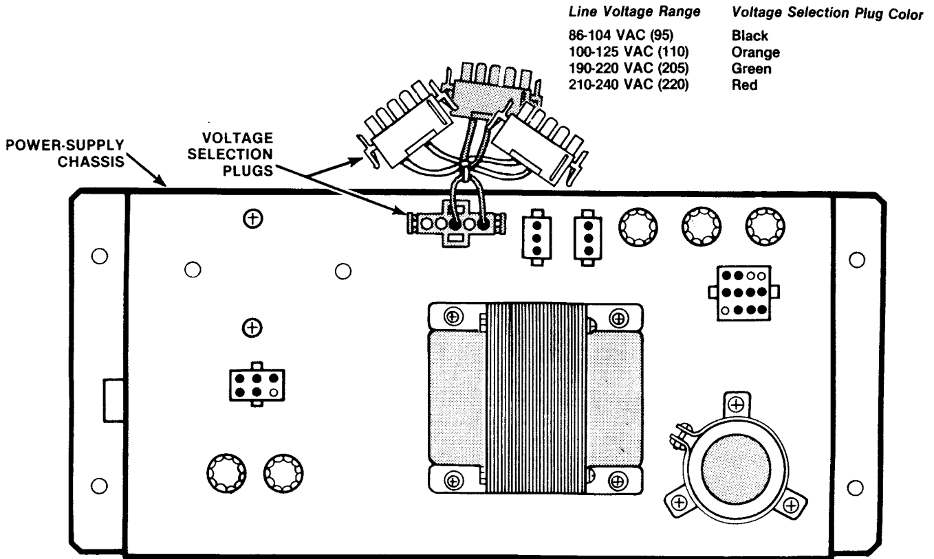
Figure 3 Power Supply
