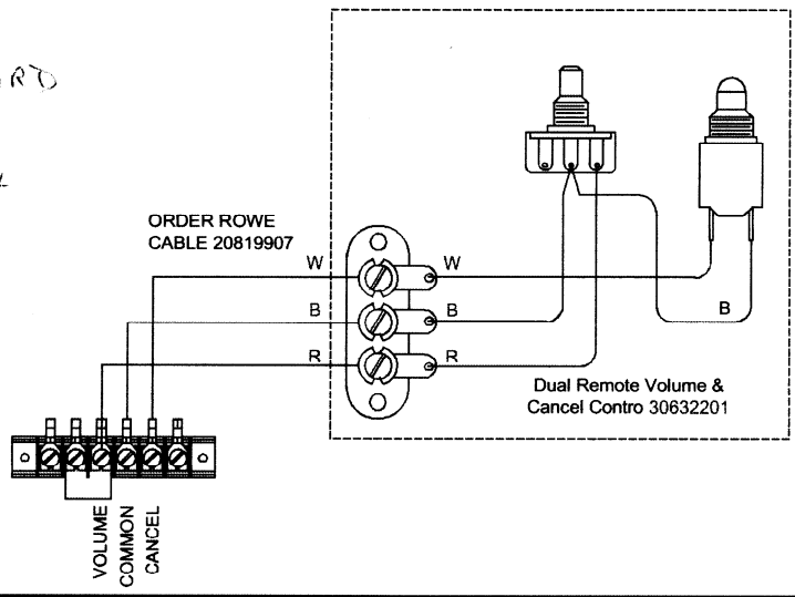
Figure 2-8A. Remote Volume Control Diagrams
