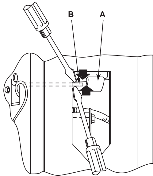
Figure 3-15. Bill Stop Flipper Adjustment
