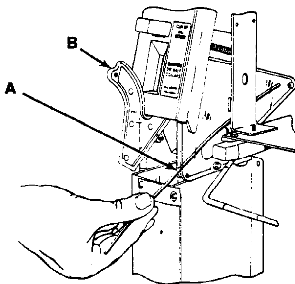
Figure 3-3. Cleaning the Coin Inlet
