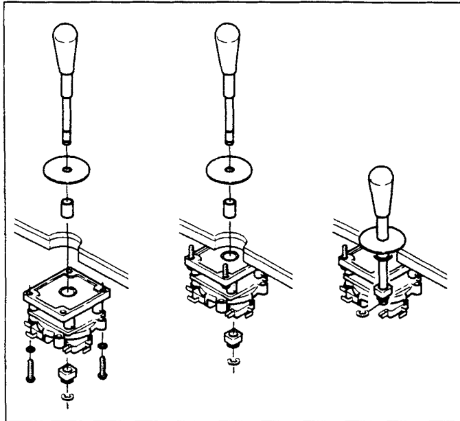
FIGURE 4 Joystick Installation
