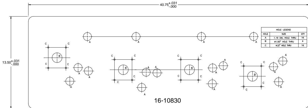
PLAYER PANEL TEMPLATE 16-10830
