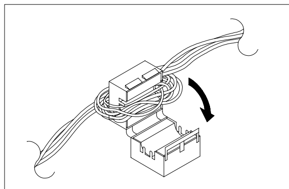
LOOP VIDEO CABLE THROUGH BEAD
