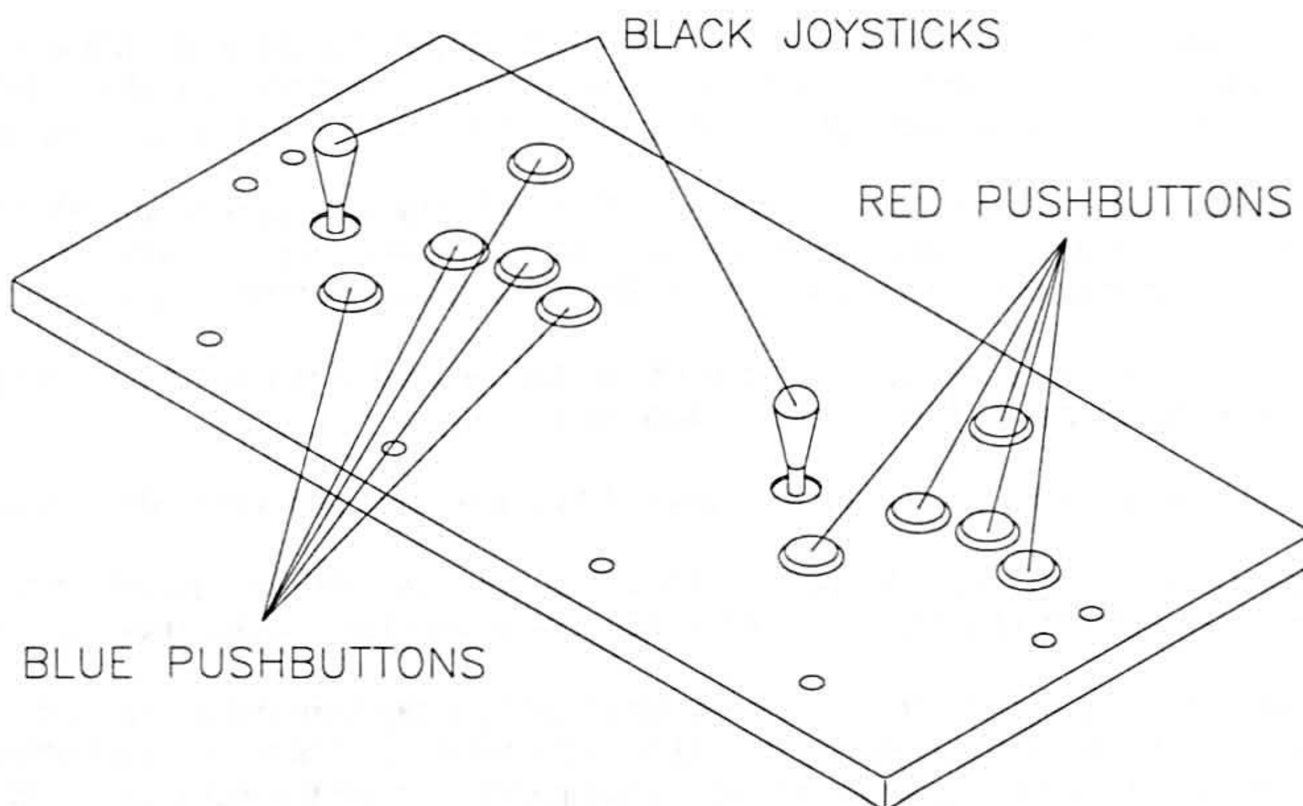
TYPICAL COMPLETED CONTROL PANEL
