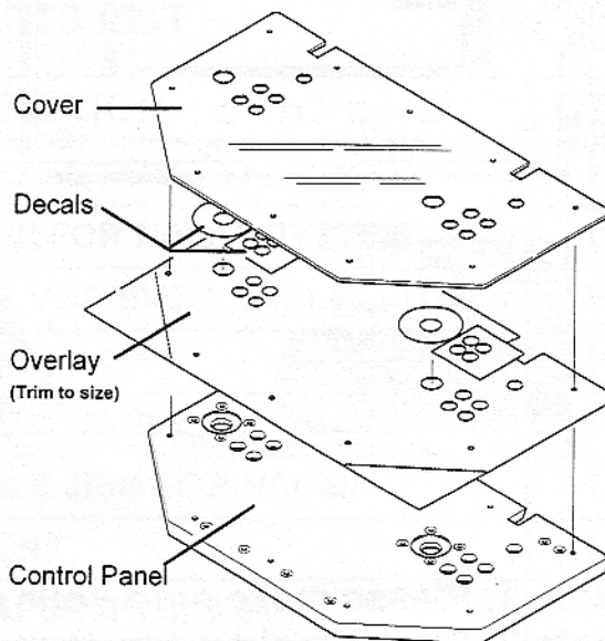
Figure 1: Overlay Installation
