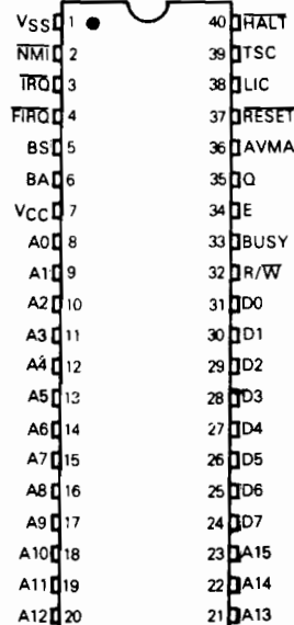
FIGURE 1 — PIN ASSIGNMENT
