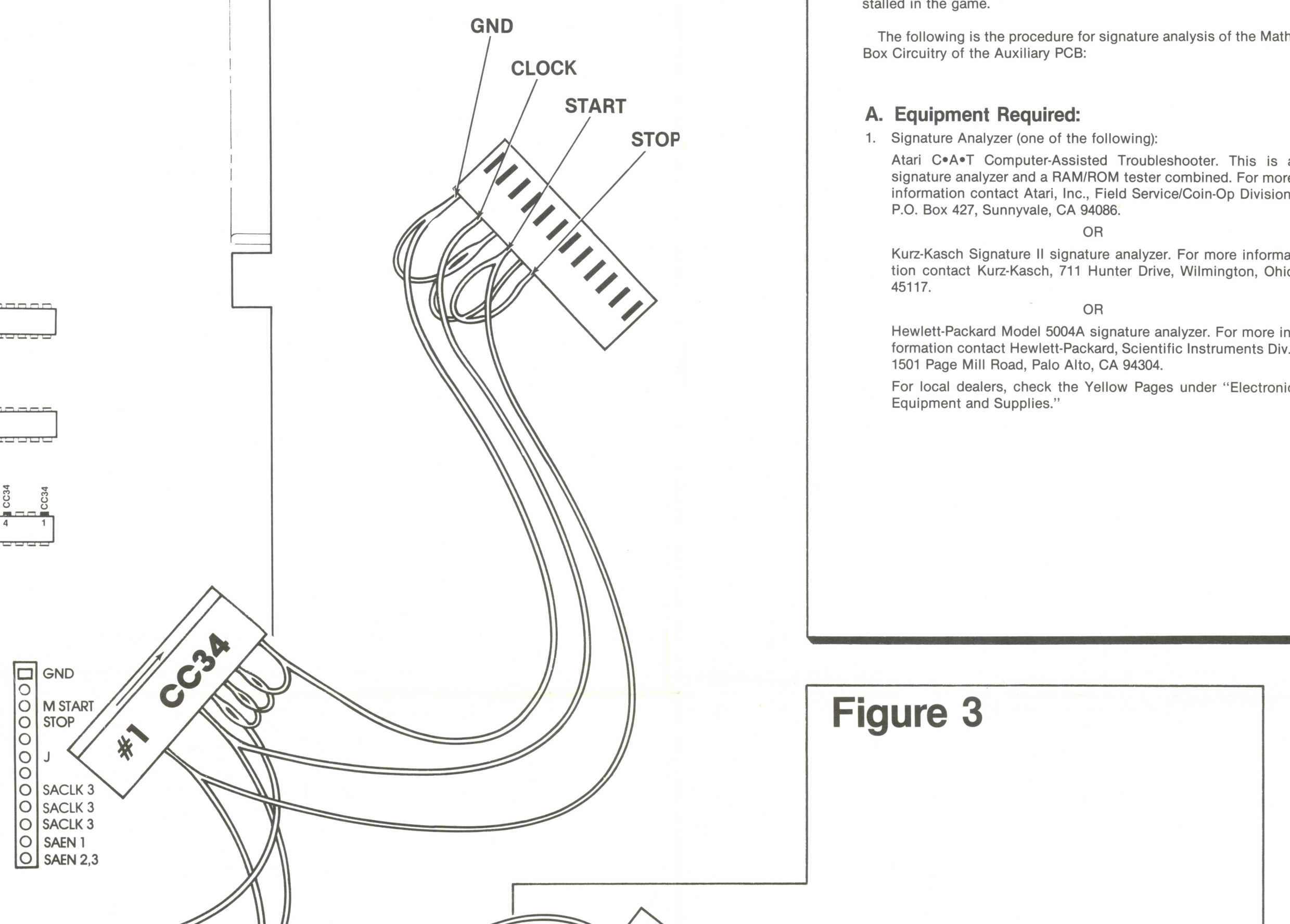
PORTION OF AUXILIARY PCB
